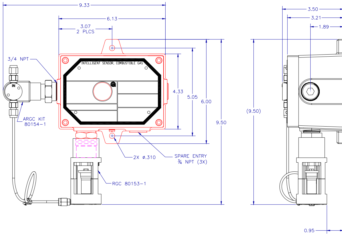
Figure 7: ARGC (80154-1 & 80153-1) with S400CH Dimensions and Outline Drawing
