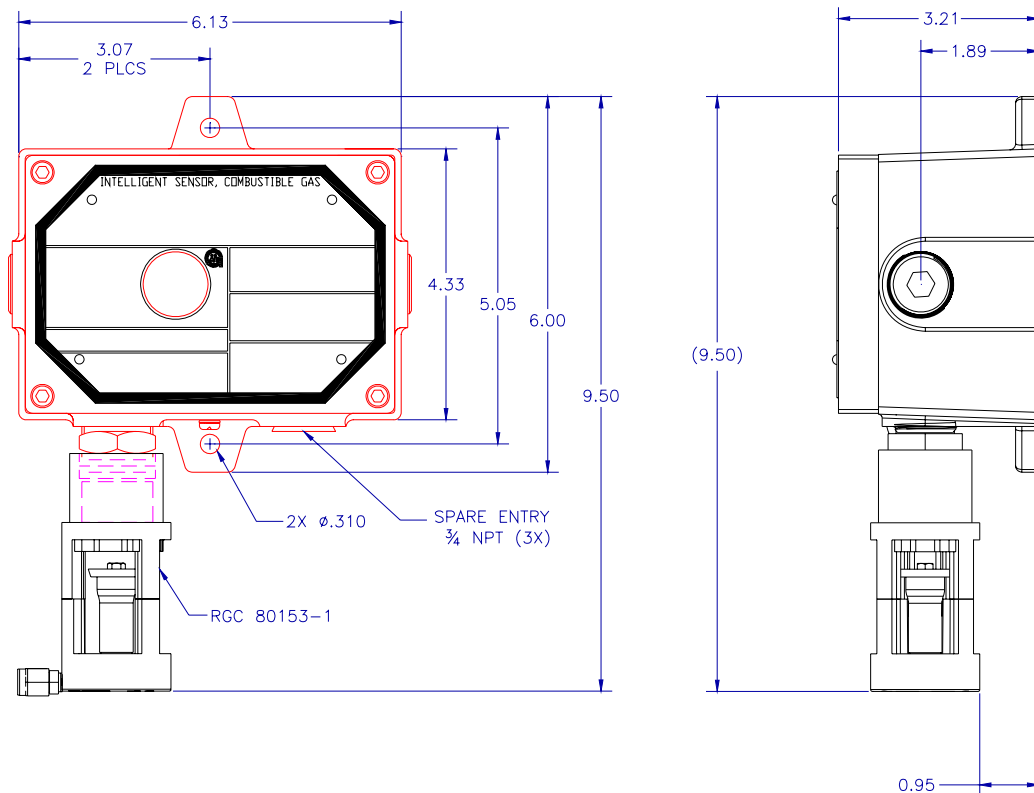
Figure 6: RGC (80153-1) with S4000CH Dimensions and Outline Drawing
